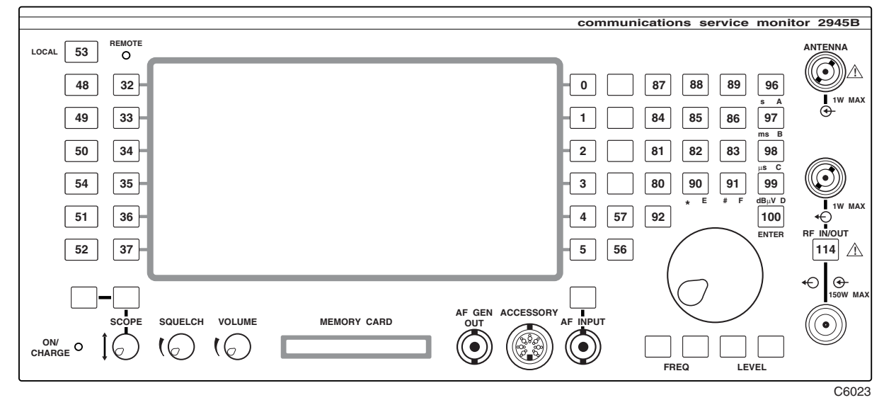
Fig. 2-4 Key code number definition
